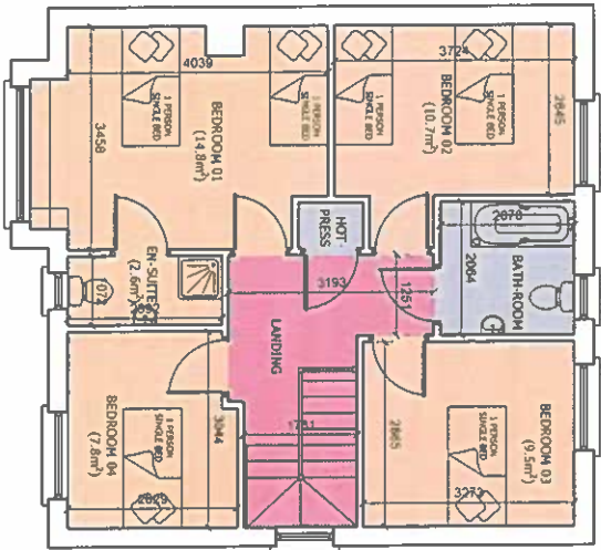
FIRST FLOOR PLAN Scale 1:125
