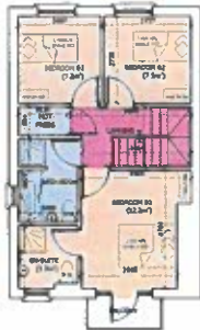
FIRST FLOOR PLAN Scale 1:125
