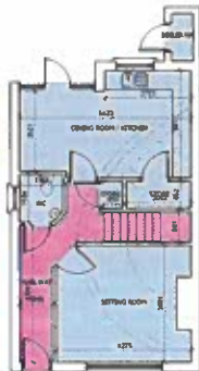
GROUND FLOOR PLAN Scale 1:125
