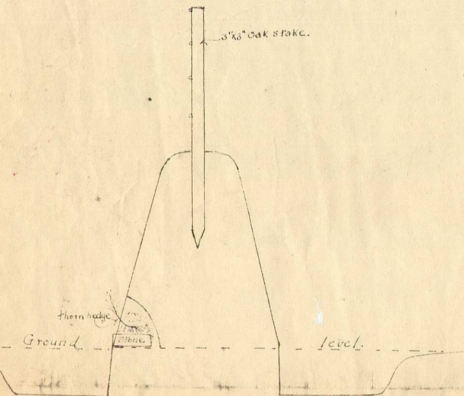
Section through Sod Fence
