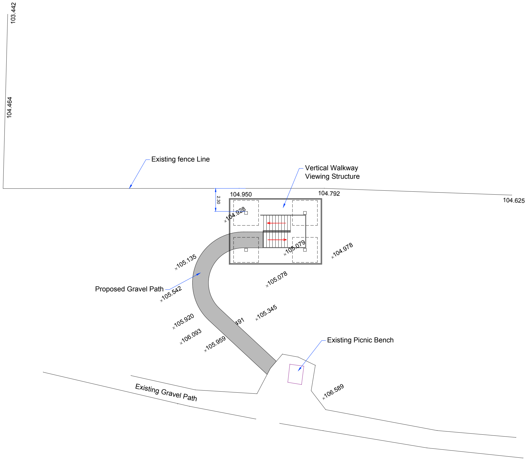
Site Plan Scale 1:100 @ A1
